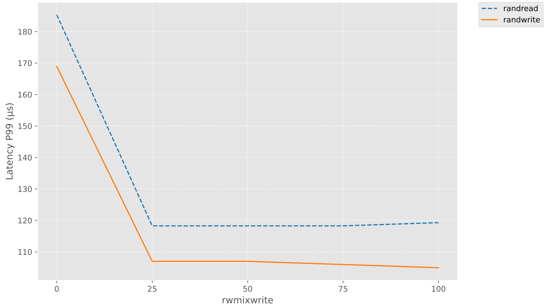
Latency P99 vs rwmixwrite
